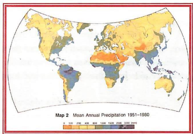
Fig. 1: Mean annual precipitation (UNEP, 1997)
