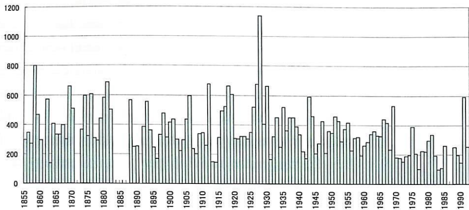
Fig. 2: Annual variability of the precipitation (Saint-Louis, Senegal)
