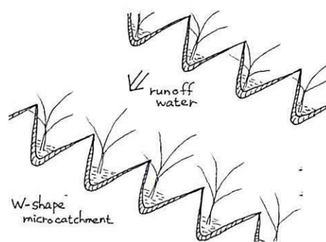
Fig. 17: An arrangement of W-shape MC
